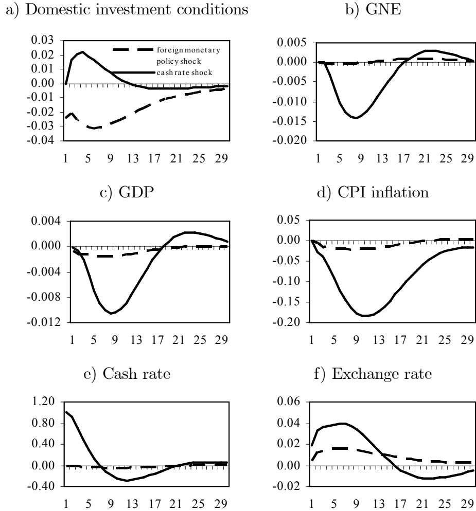
Figure 2: Impulse responses to a domestic and global monetary policy shock
