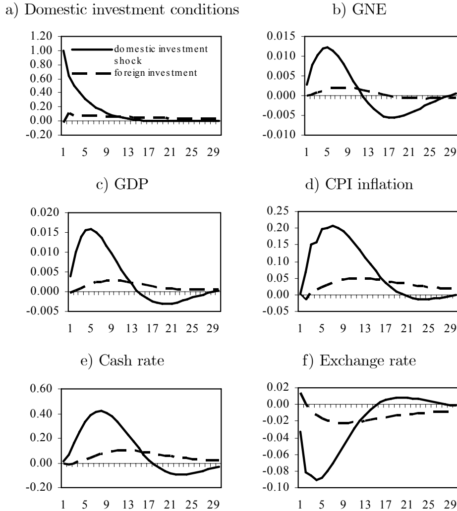
Figure 3: Impulse responses to a domestic and global investment conditions shock
