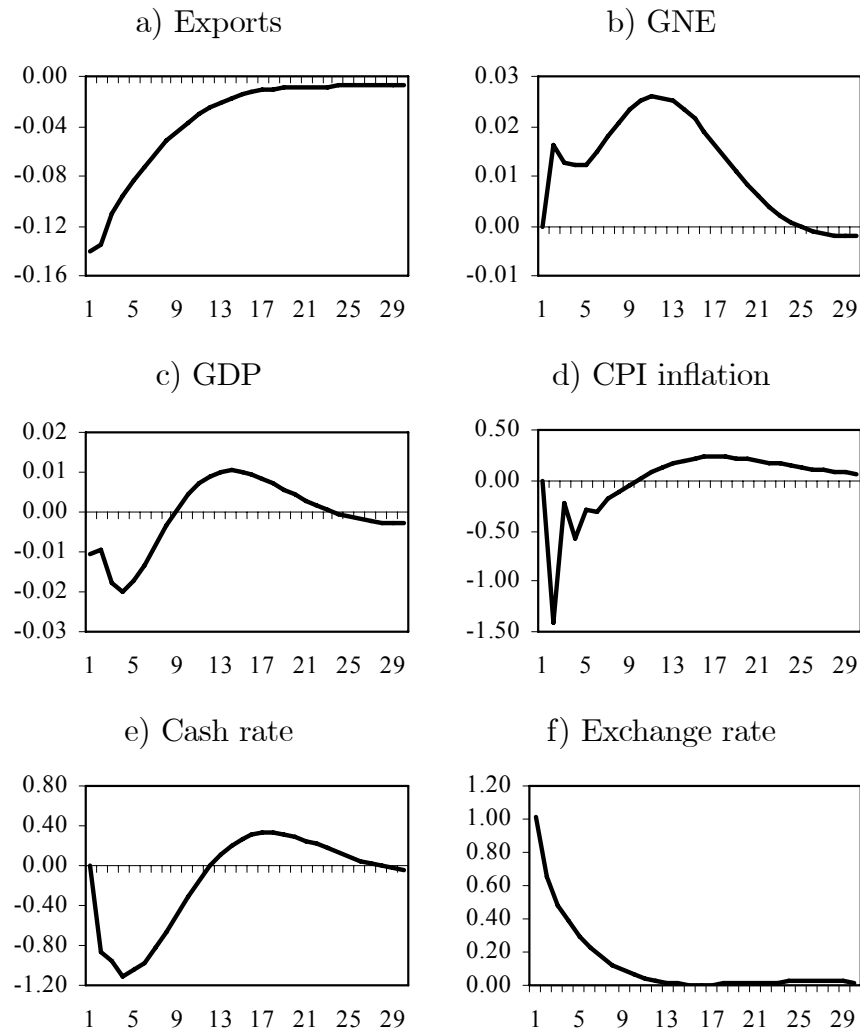
Figure 4: Impulse responses to an exchange rate shock
