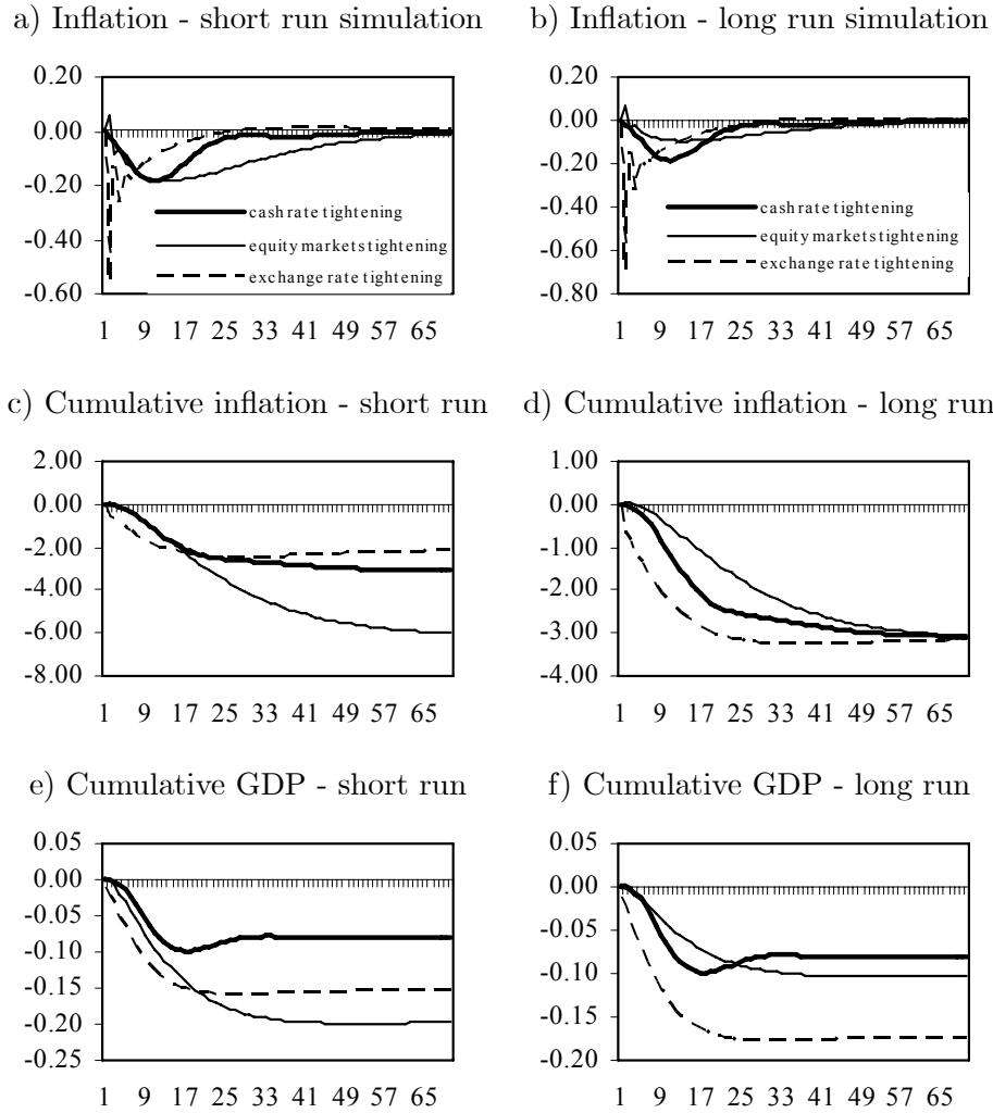
Figure 7: Impulse responses of inflation, cumulative inflation and cumulative GDP to alternative monetary policy shocks
