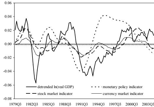
Figure 6: Monetary policy, equity market and exchange rate effects
