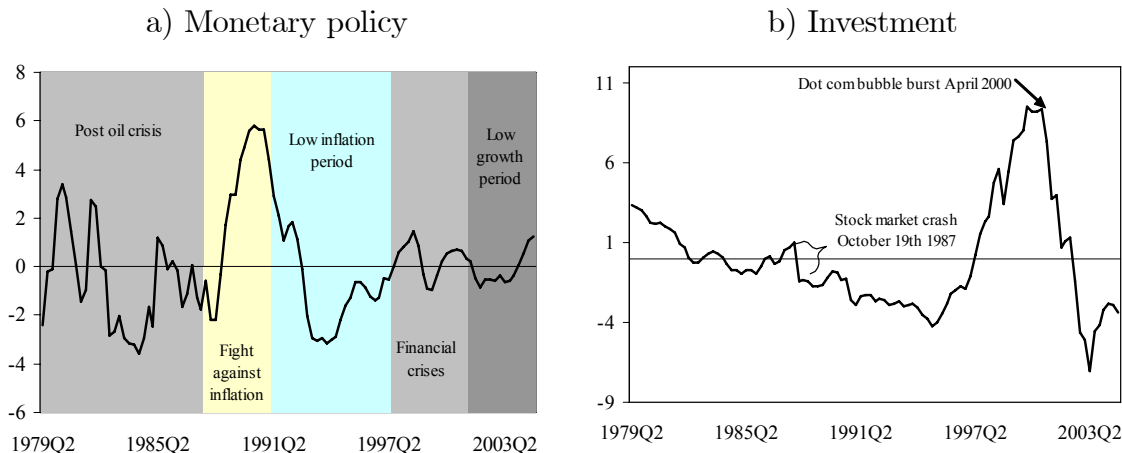
Figure 1: Global monetary policy and investment conditions
