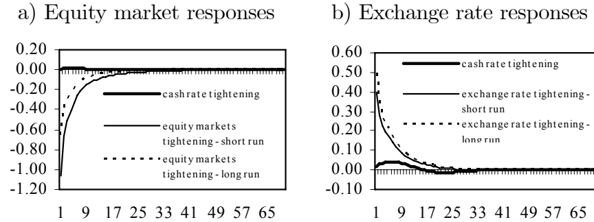
Figure 9: Responses of equity and exchange rate markets to alternative policy shocks.
