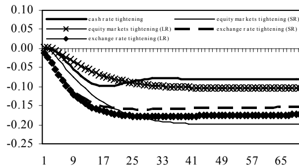
Figure 8: Cumulative impulses of GDP - all experiments
