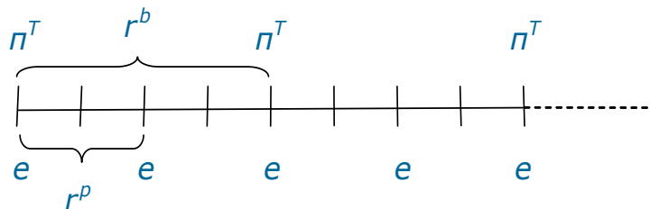
FIGURE 1. An example of the timing with r^b = 4 , r^p = 2 showing two repetitions of the dynamic stage game (the short-run policy instrument \pi(i) adjustable every period has been left out for clarity).
